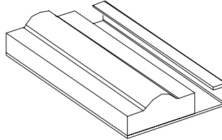
GUIDE RAIL W/ ANTI-TIP CHANNEL
